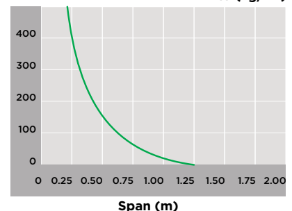
Cantilever Support
