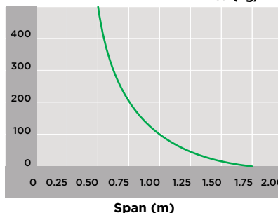
Continuous Support
