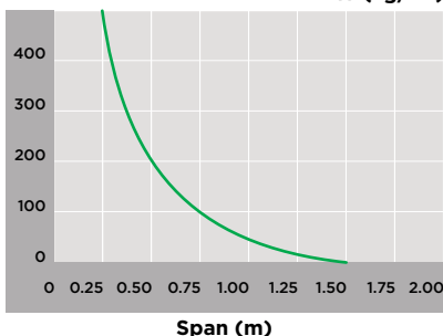
Simple Support
