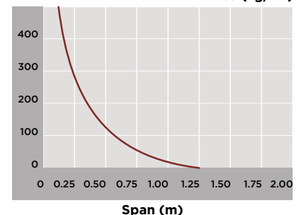
Cantilever Support
