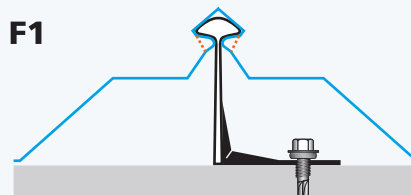
Middle tight frame SF-750
