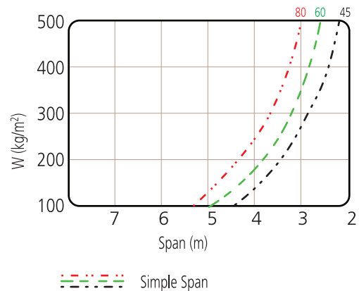
Simple support
