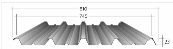
GG-750 Thickness: 30-60 Bj.L.S Minimum Length: 0.80 m Maximum Length: 12 m
