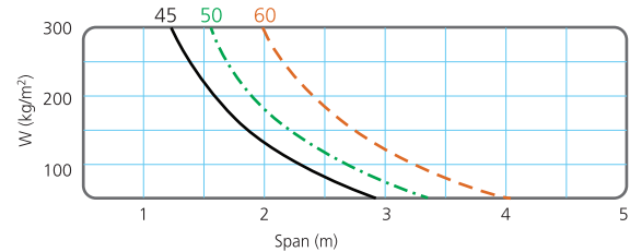
Simple support
