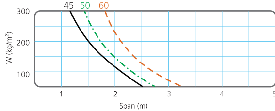
Continuous support
