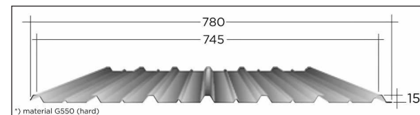
A-750 Thickness: 20-25 Bj.L.S Minimum Length: 0.80 m Maximum Length: 12 m
