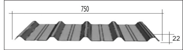
GH-750 Thickness: 30-50 Bj.L.S Minimum Length: 1.50 m Maximum Length: 12 m
