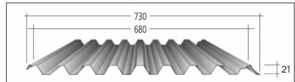
G-680 Thickness: 30-60 Bj.L.S Minimum Length: 0.80 m Maximum Length: 12 m
