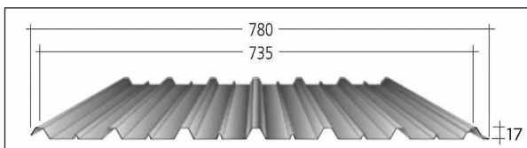
A-735 Thickness: 20-60 Bj.L.S Minimum Length: 0.80 m Maximum Length: 12 m
