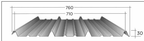
F-714 Thickness: 40-60 Bj.L.S Minimum Length: 0.80 m Maximum Length: 12 m
