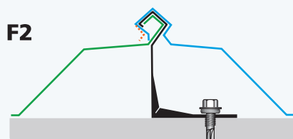
Overlap tight frame SF-750
