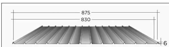
B-832 Thickness: 20-60 Bj.L.S Minimum Length: 0.80 m Maximum Length: 12 m
