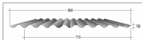
C-710 Thickness: Hard : 20-30 Bj.L.S Soft : 30-120 Bj.L.S Minimum Length: 1.50 m Maximum Length: Hard : 3.65 m (for 20 Bj.L.S) Soft : 3.65 m
