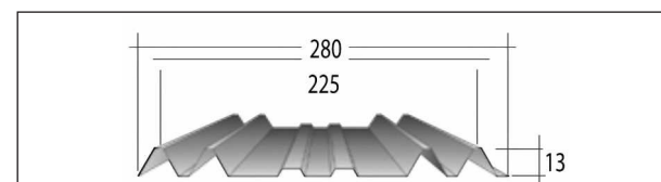
H-225 Thickness: 20-60 Bj.L.S Minimum Length: 0.80 m Maximum Length: 5 m
