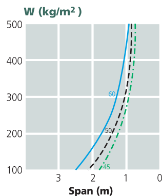
Overlap tight frame SF-750
