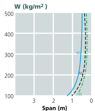
Cantilever support
